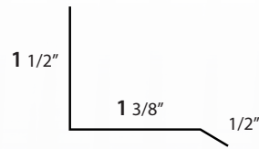
WINDOW CAP
