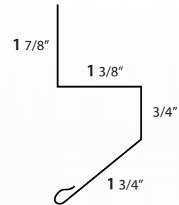
RAT GUARD
