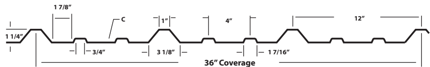
PBR PROFILE
