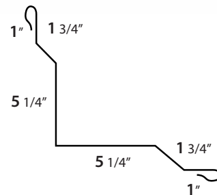
TOP FINISHER
