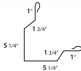
CORNER
