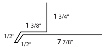
TOP FINISHER
