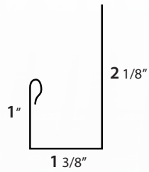
J TRIM
