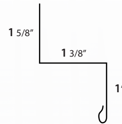
DOUBLE ANGLE
