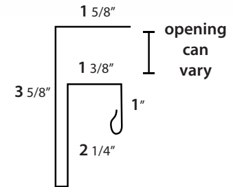
DOUBLE J
